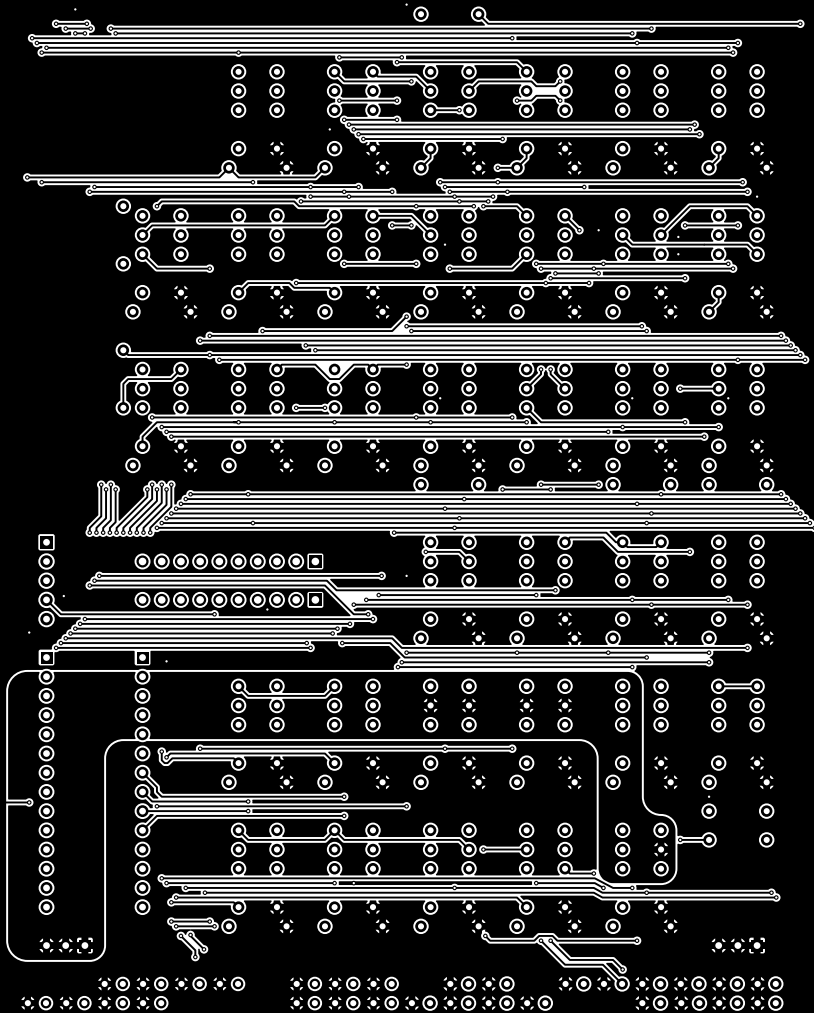
W2 BACKPLANE CONTROLLER CARD : GOTO & MOV8/16
