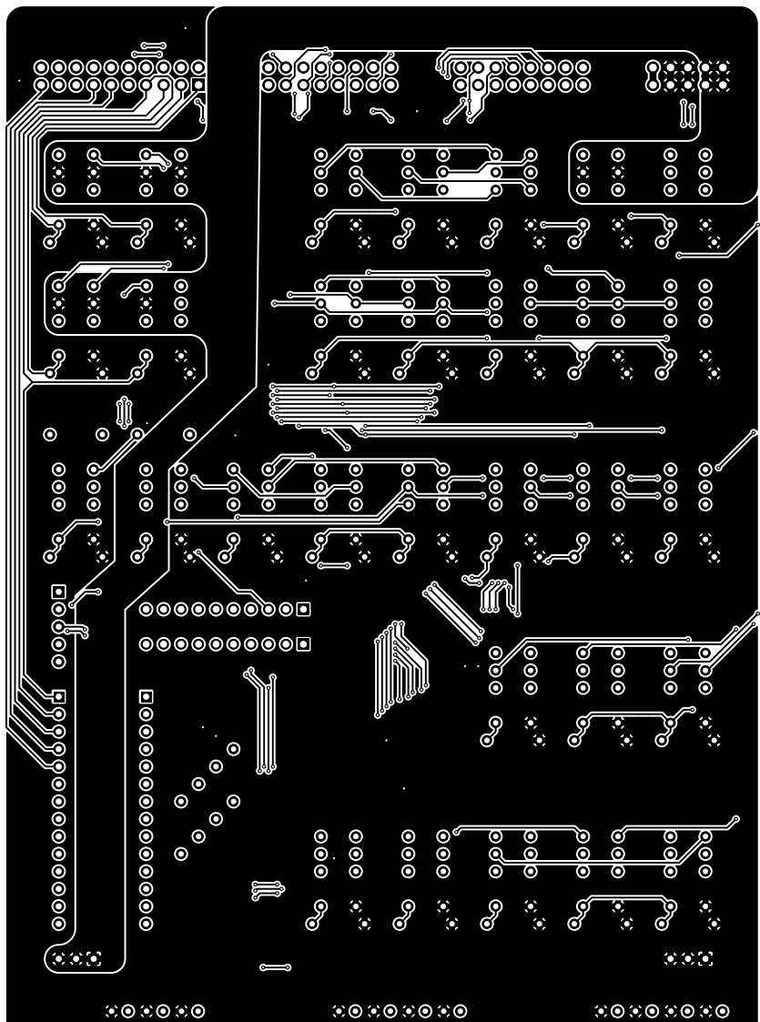
W1 BACKPLANE CONTROLLER CARD : ALU, LOAD, STORE & SETAB
